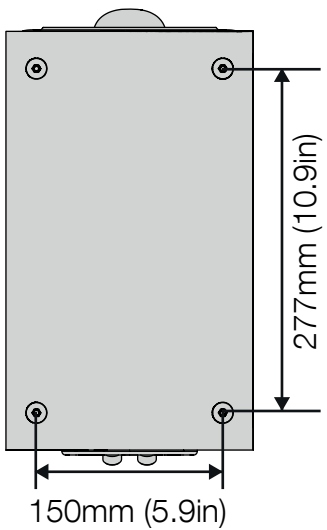
CABINET BASE SCREW ALIGNMENT FOR PLINTH
