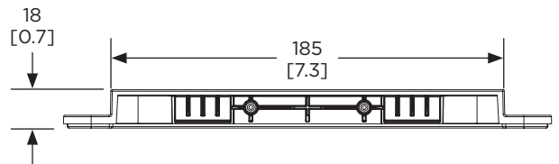
Rear View
